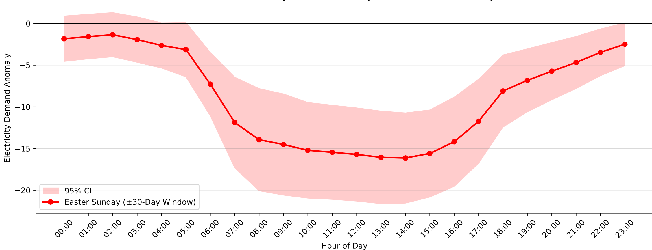
Gore Hill Demand Anomaly: Easter Sunday (2004-2017, \pm 30 -Day Window)
